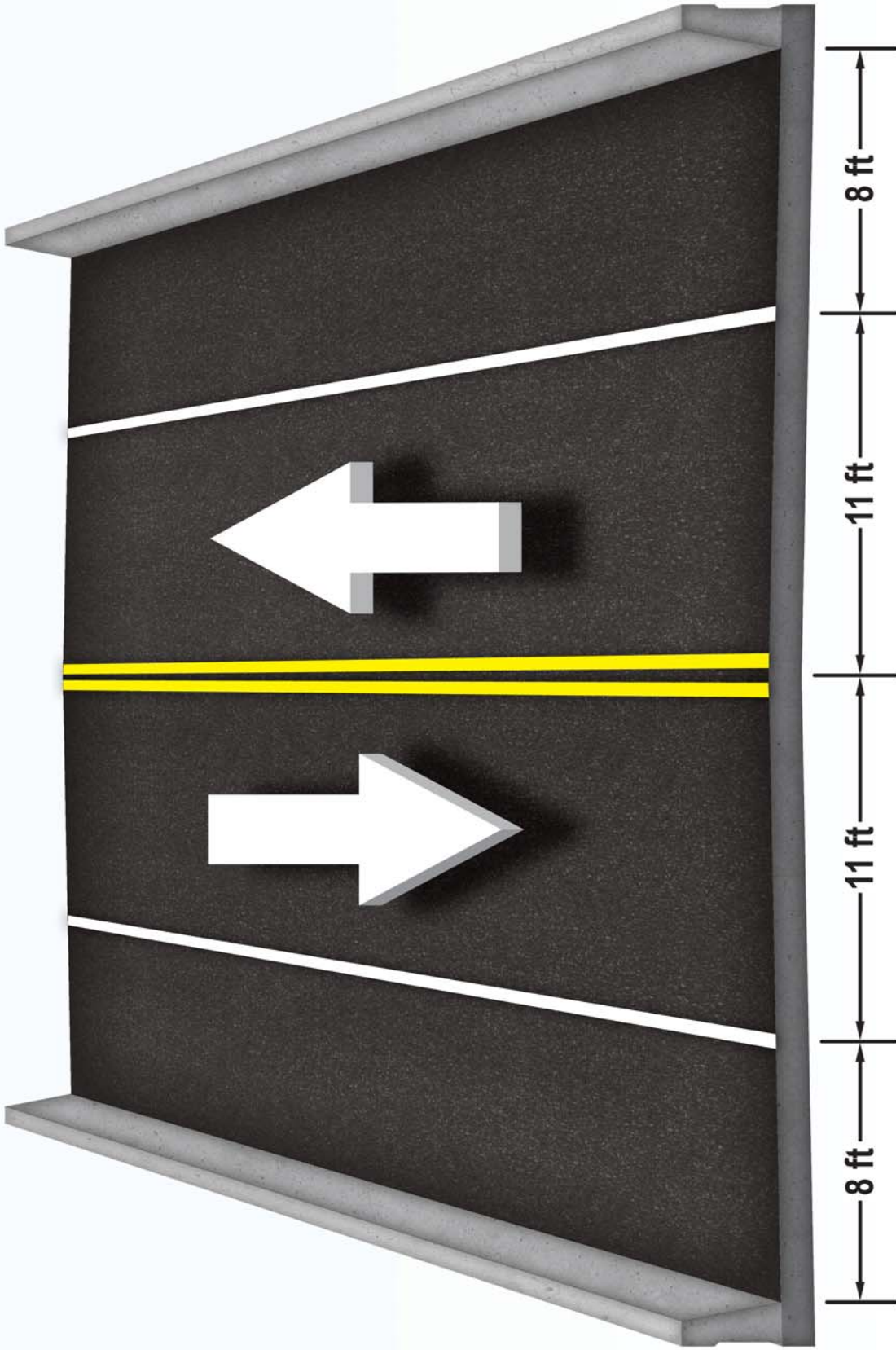
Proposed Bridge Typical Section 180th Street over Little River Bridge Replacement
