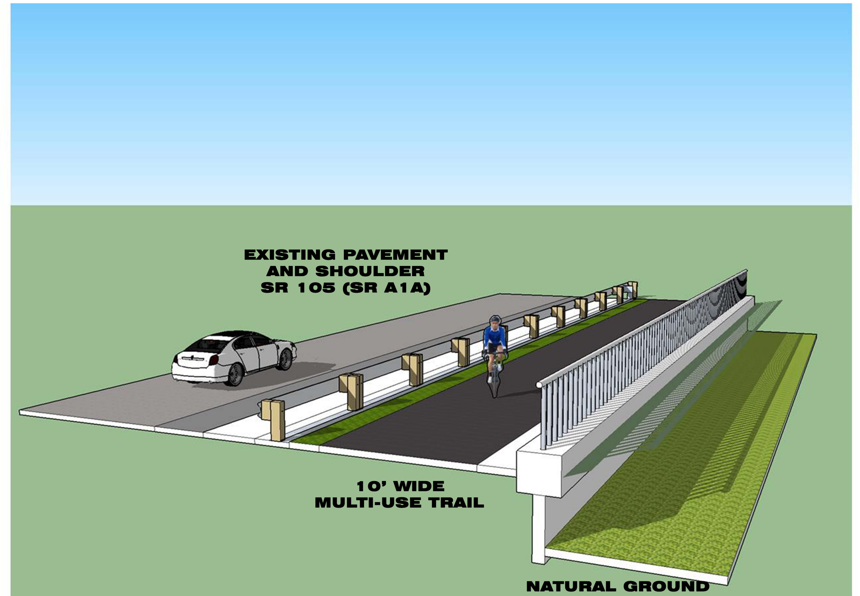
PROPOSED MULTI-USE TRAIL WITH WALL
