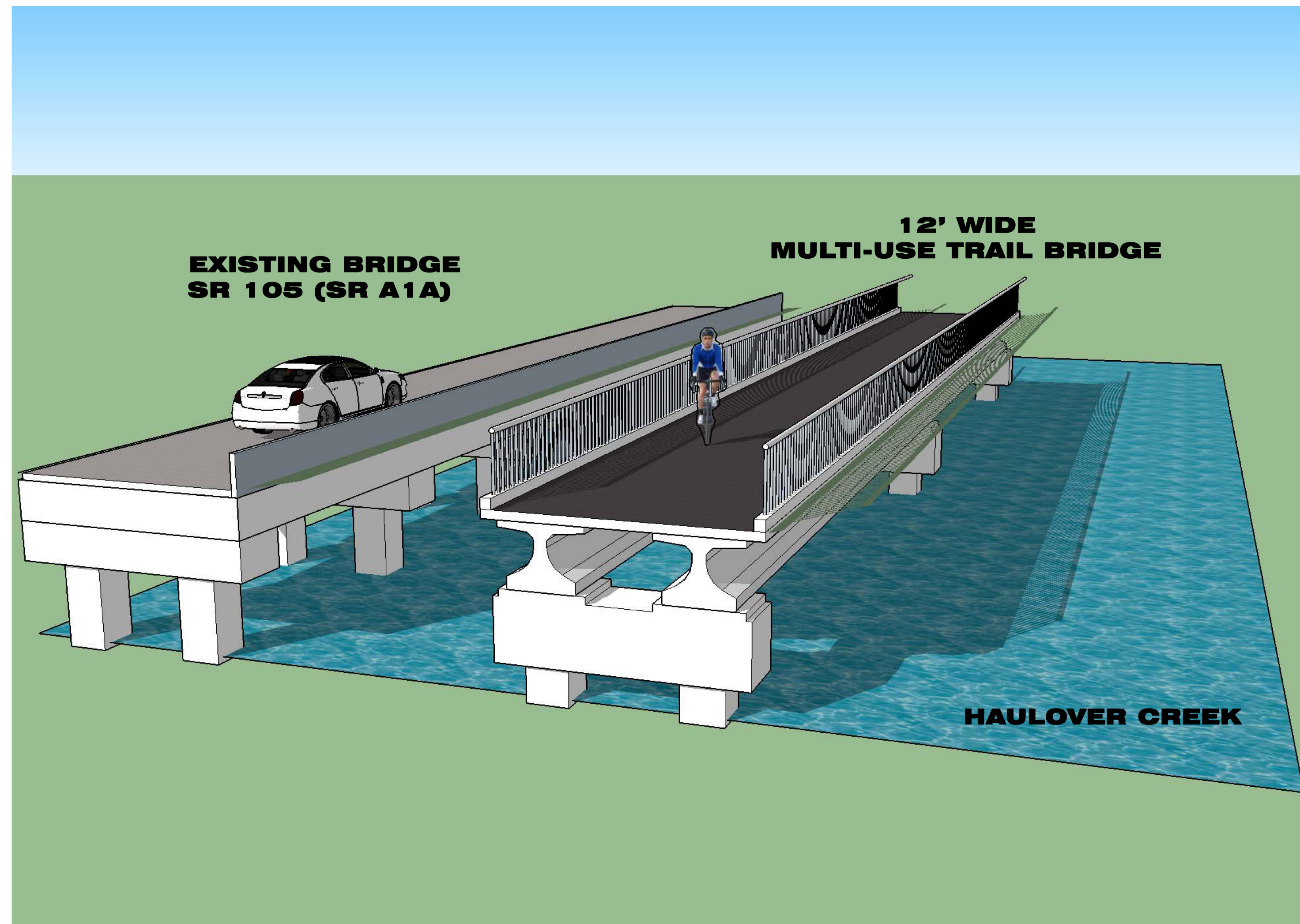
PROPOSED MULTI-USE TRAIL BRIDGE
